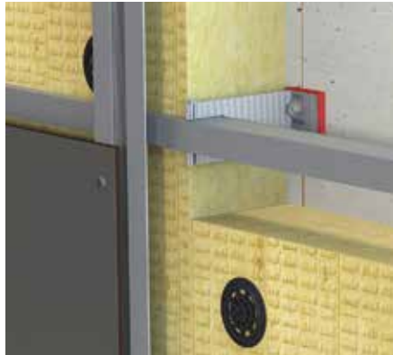
2-lagiges System
